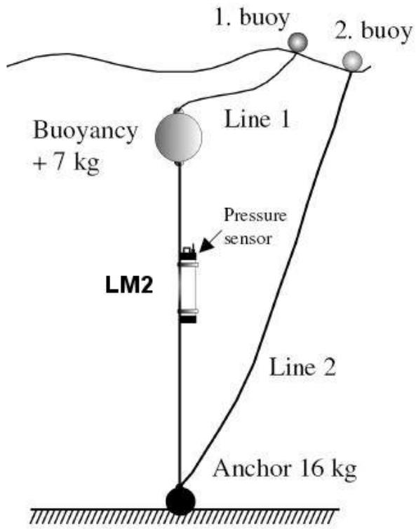
Typical installation for wave height measurements
